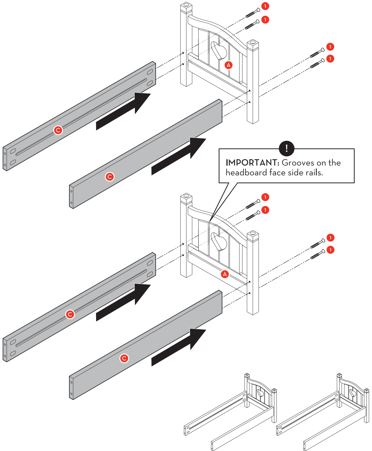
Assembled View
